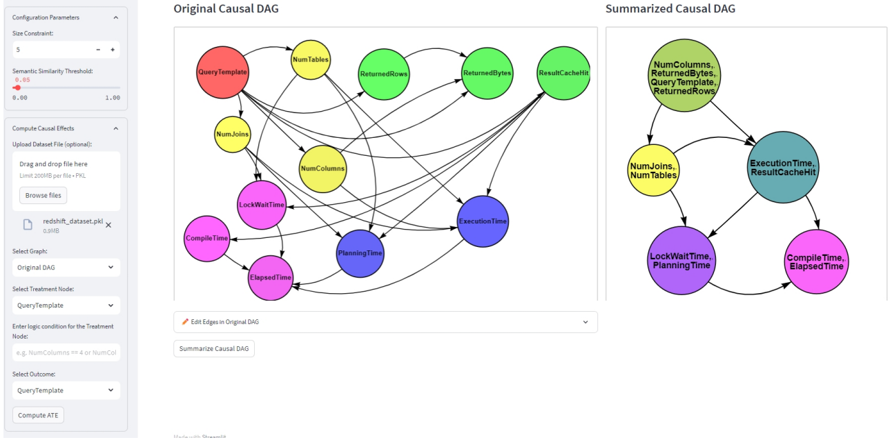
Figure 1: CAUSALENS UI showing example causal DAGs for analyzing the Redshift dataset on query performance. Left: Manual causal DAG with color-coded semantic relationships. Right: Generated summary causal DAG based on user-defined size and similarity constraints.
